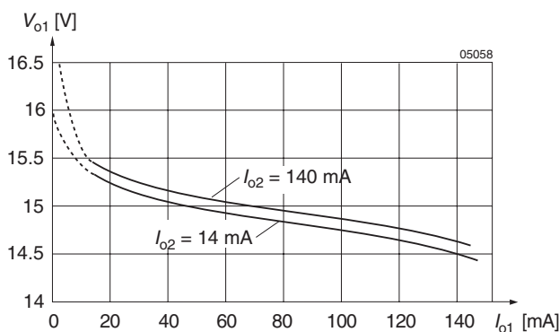
Fig. 10 Cross load regulation of dual output units. U_{o1} versus I_{o1} (typ) for various I_{o2} (48IMS6-1515-9).
