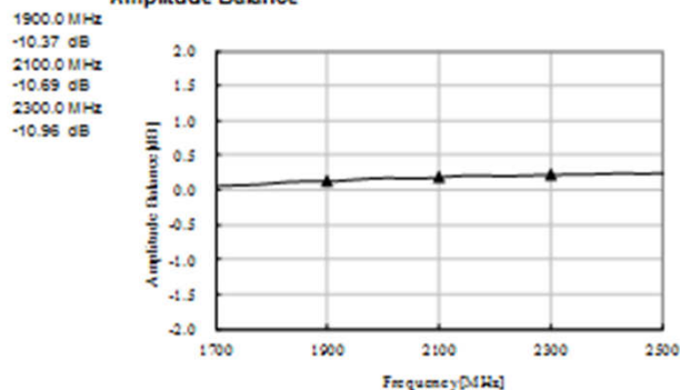
Amplitude Balance
