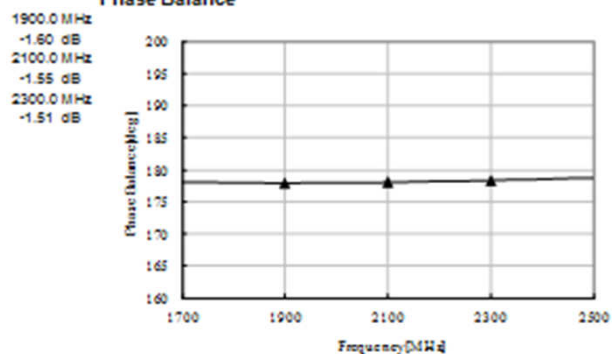
Phase Balance
