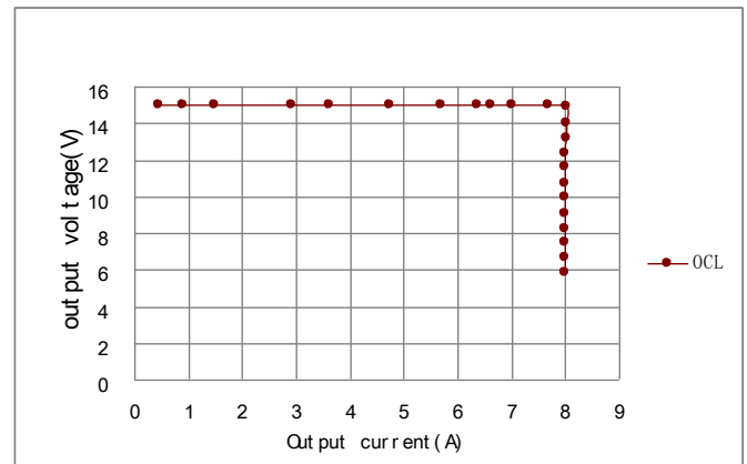
Figure 11: Output voltage vs. load current showing typical current limit curves and converter shutdown points.
