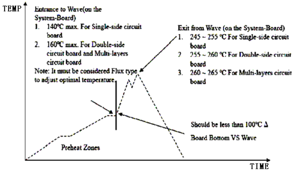
Figure 20 recommended temperature profile for lead-free wave soldering
