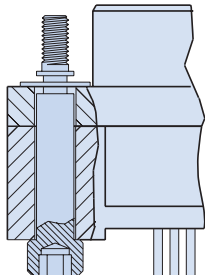
M Style Hex Head Jackscrew with E-Ring
