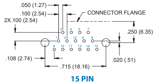
15 PIN
