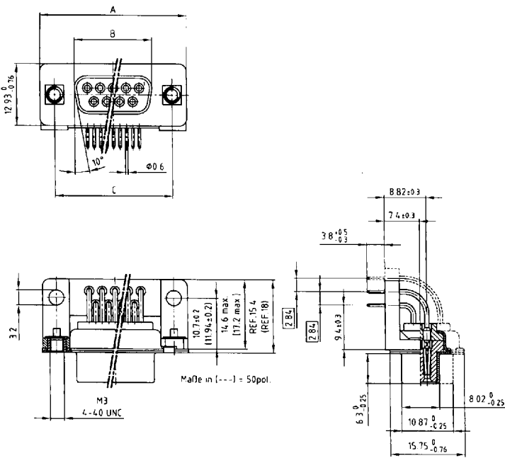
Socket connector
