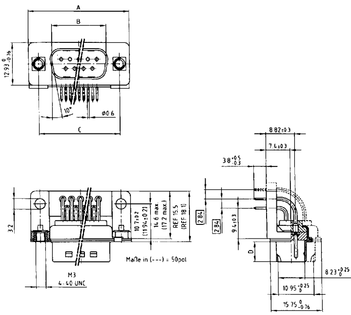
Plug connector
